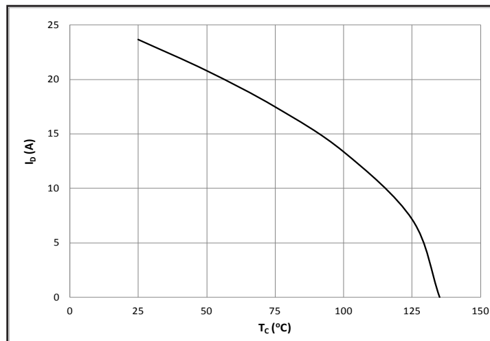
Figure 10. Continuous Current Derating Curve
