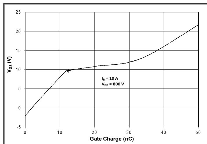
Figure 12. Typical Gate Charge Characteristics (25°C)
