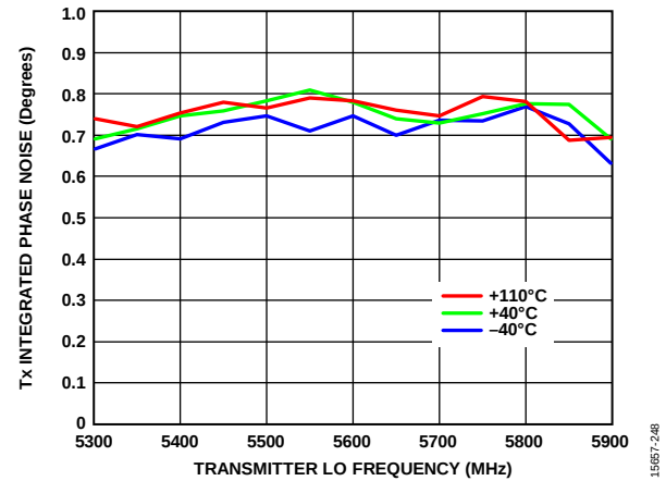
Figure 209. Tx Integrated Phase Noise vs. Transmitter LO Frequency, 75 MHz RF Bandwidth, CW 10 MHz Offset from LO, 3 dB Digital Backoff
