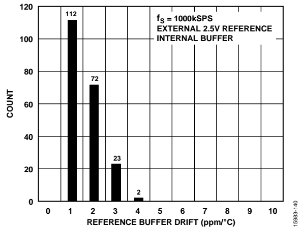
Figure 16. Reference Buffer Drift, External 2.5 V Reference
